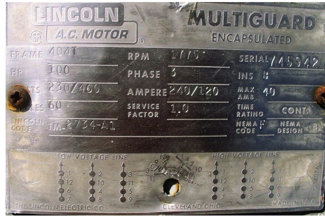
Figure 3. Nameplate of a dual voltage motor with high and low voltage wiring diagrams.
