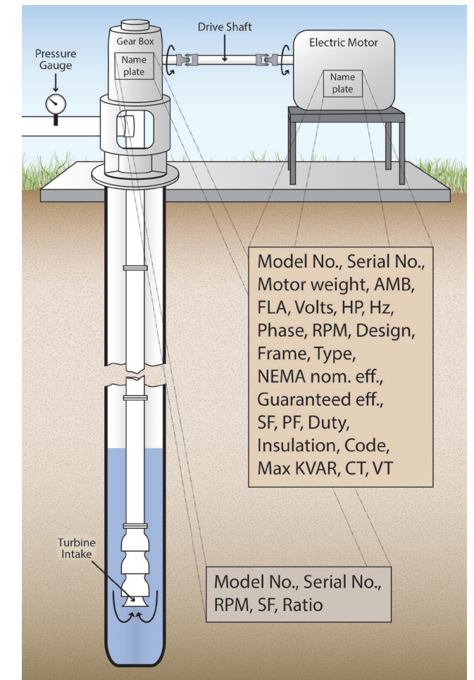
Figure 1. Common nameplate information found on gear-head housings and AC motors.
