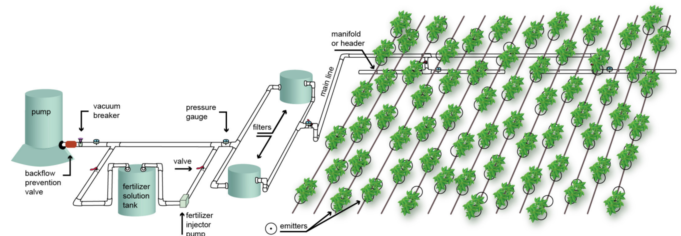
Figure 1. Typical drip irrigation system layout.
