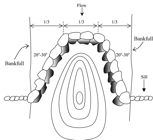
Figure 7. Constructed rock riffle and rock cross-vane.
