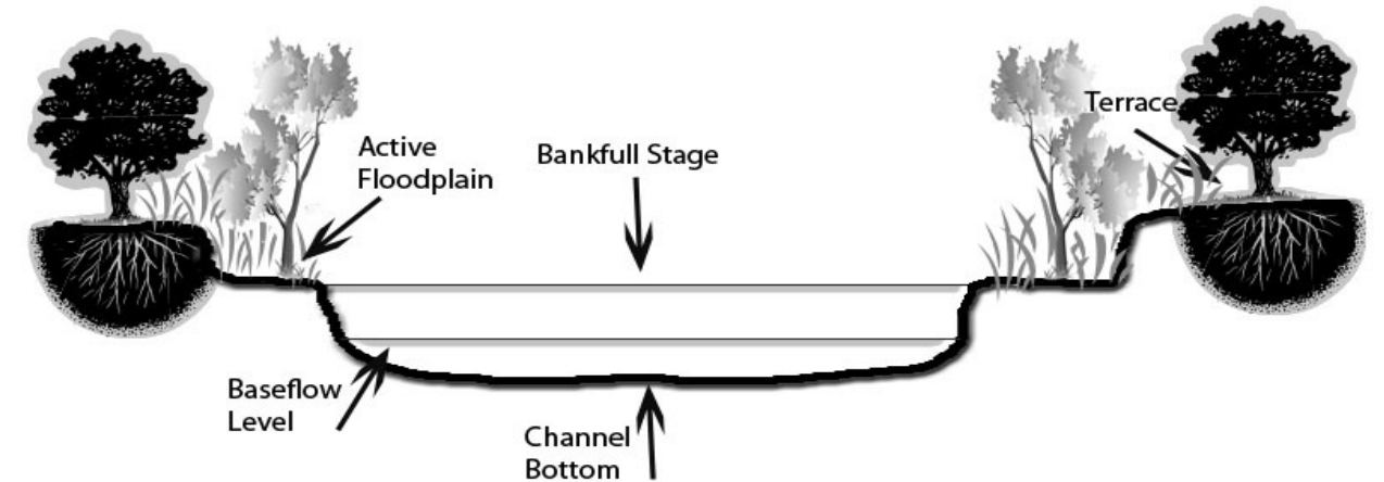
Figure 1. Cross-section of stream corridor with major components labeled.
