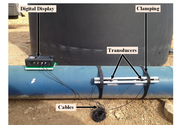
Figure 1. Ultrasonic flowmeter installed on a pump outlet pipe.
