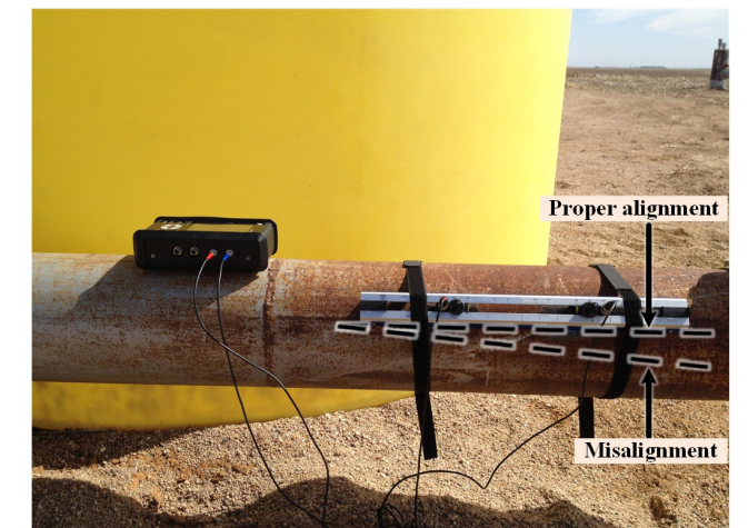
Figure 7. Alignment of transducers.
