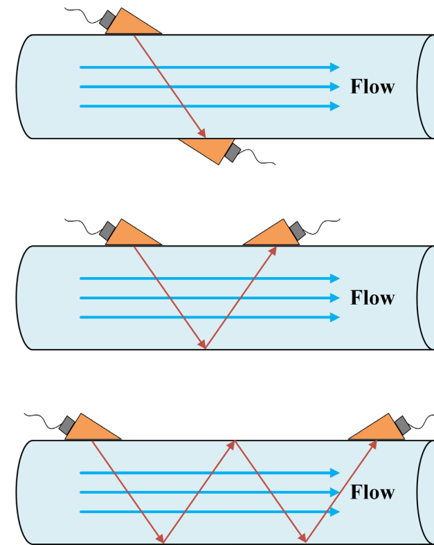
Figure 6. Common mounting configurations: Z method (top), V method (middle) and W method (bottom).
