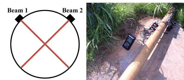
Figure 3. Example of cross beam measurement (left) and use of two flowmeters to verify measurements (right).
