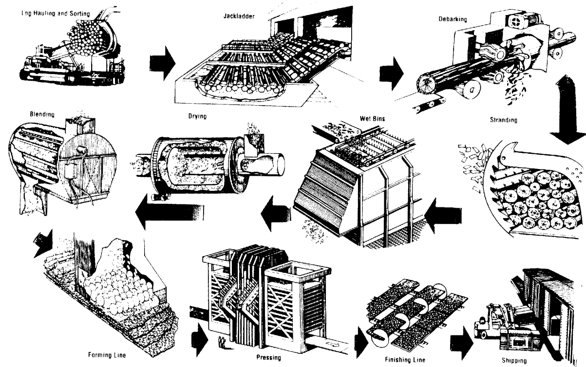
Figure 2. A general flow chart of OSB production. From J. Lowood. Oriented Strand Board and Waferboard. 1997. Engineered Wood Products. PFS Research Foundation.
