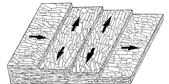
Figure 1. A schematic illustrating strand orientation of a typical OSB.
