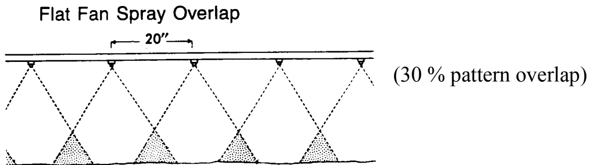
Figure 10.11. Spray Patterns From Adjacent Nozzles Must Be Overlapped To Produce Uniform Spray Coverage [Above].
