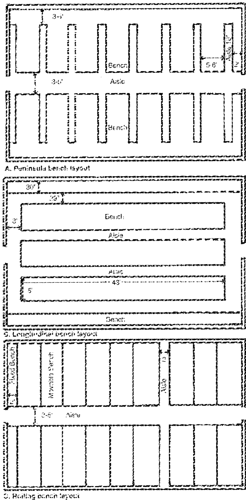
Figure 1. Greenhouse bench layouts. Design are intended for comparison only; exact dimension will vary with each greenhouse.
