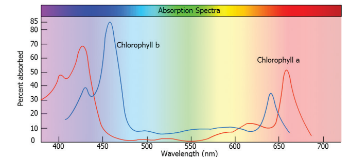
Figure 1. Spectral absorbance of chlorophyll in living leaves.
