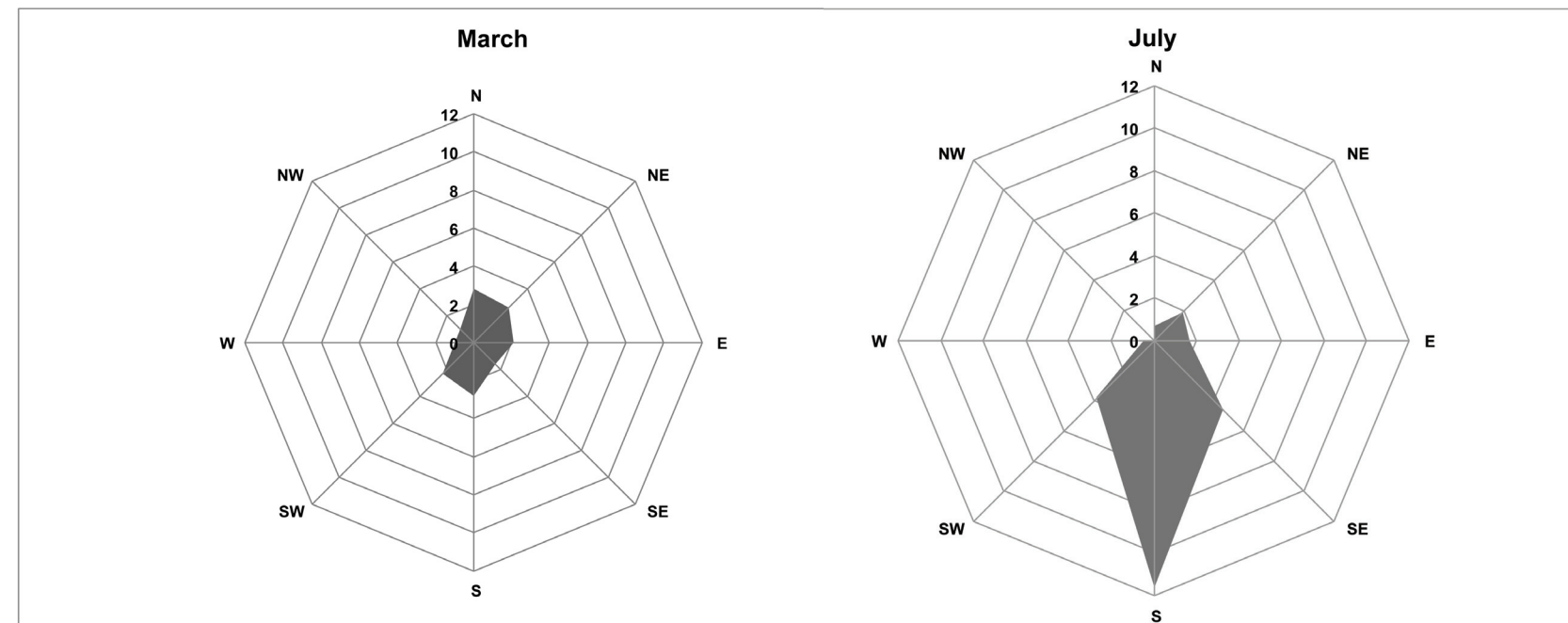
Figure 4. Average number of burn days by wind direction for March and July, demonstrating how different seasons of the year allow for more burn days and more opportunities for specific wind directions than other seasons.
