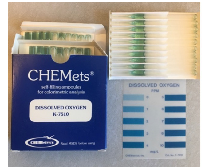
Figure 1. A relatively inexpensive chemical test kit for dissolved oxygen concentration. The ampule neck is snapped, and water is drawn up into it. A simple color comparison indicates the concentration of oxygen.
